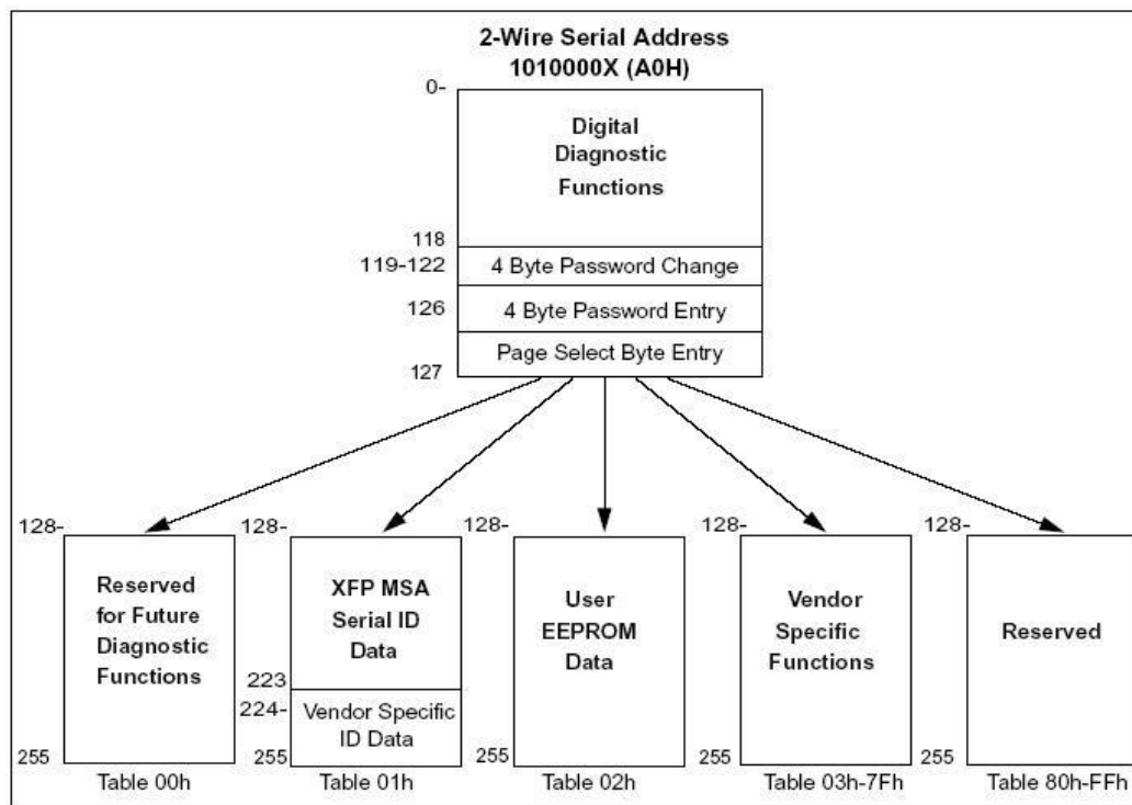
Figure4. 2-wire Serial Digital Diagnostic Memory Map
