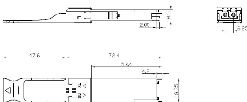
Figure 4. Mechanical Dimensions
