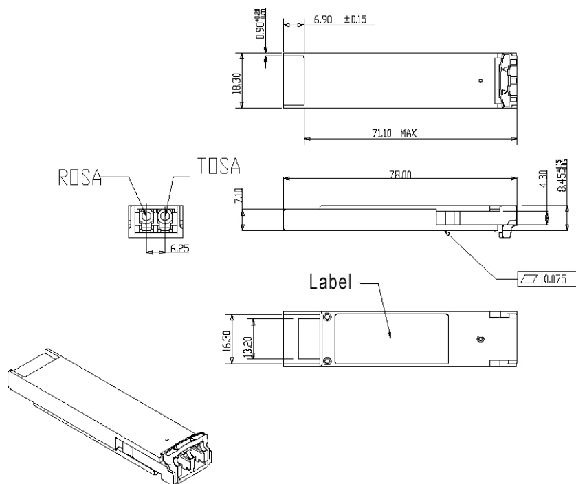
Figure3. Mechanical Specifications
