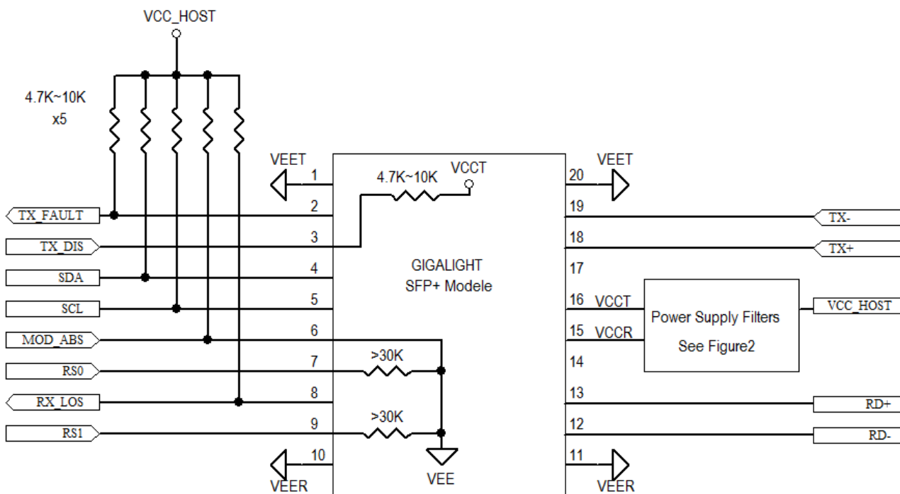
Figure3. Host-Module Interface
