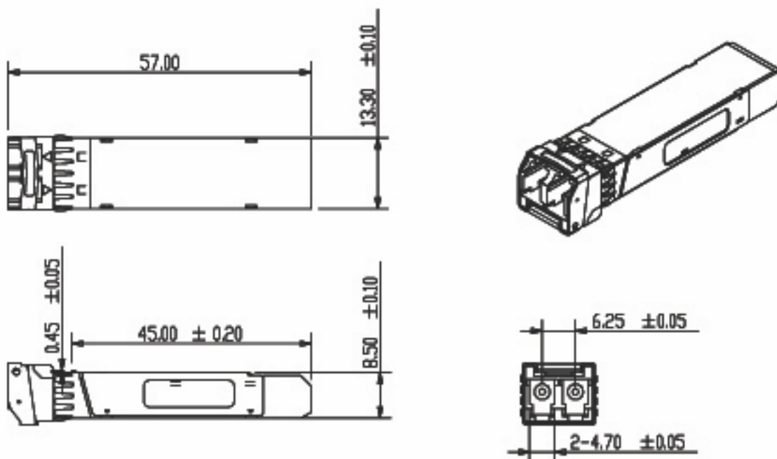
Figure6. Mechanical Specifications
