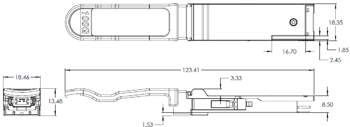
Figure 2. FTLC9152RGPL Mechanical Dimensions.
