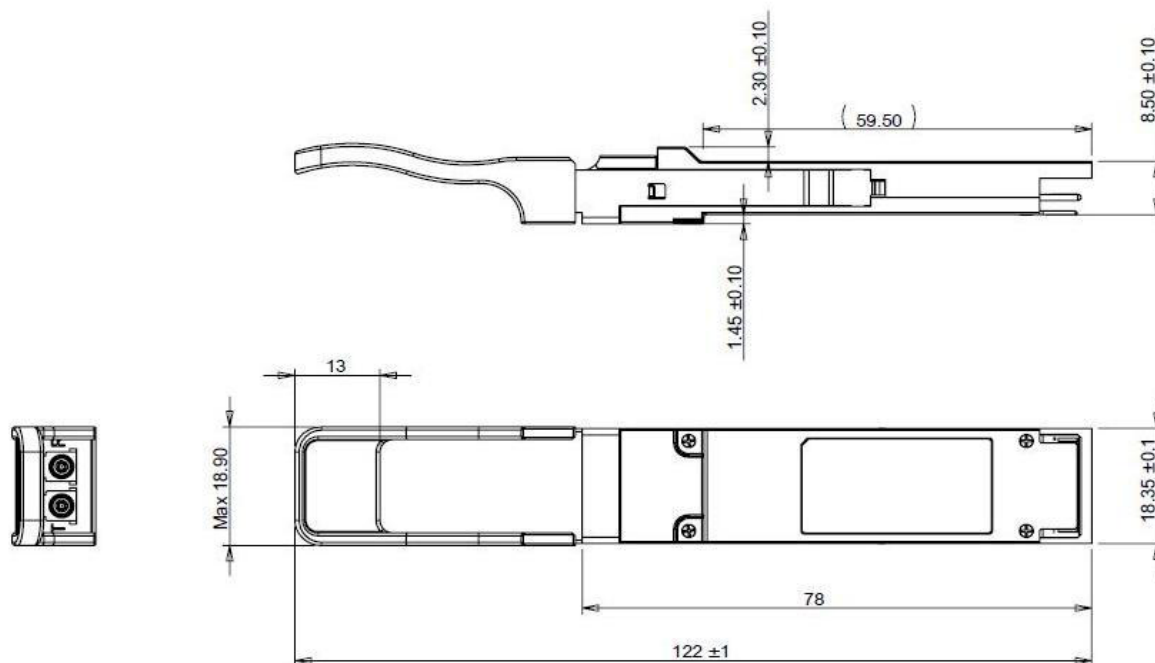
Figure 4. Mechanical Outline
