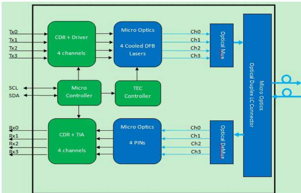
Figure 1. QSFP28 LR4 (Ethernet) Transceiver Block Diagram
