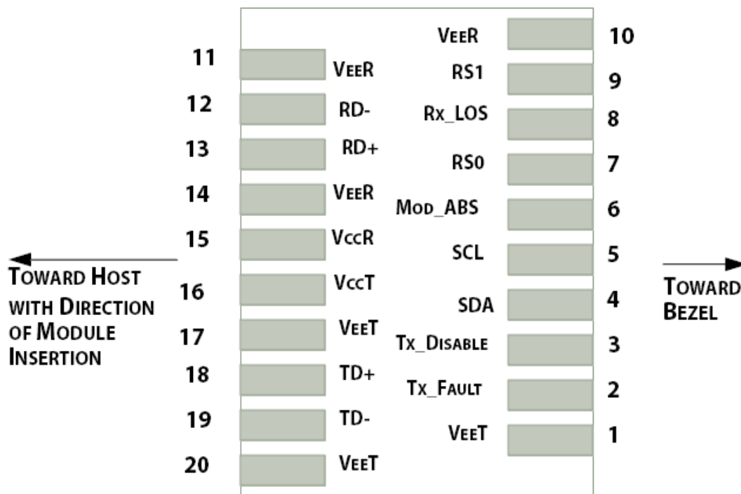
Figure1. Electrical Pin-out Details
