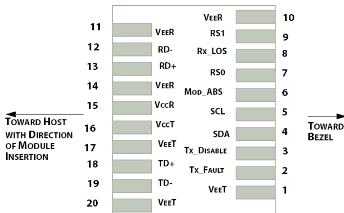
Figure1.Electrical Pin-out Details
