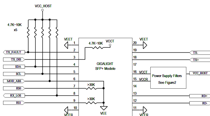
Figure3. Host-Module Interface
