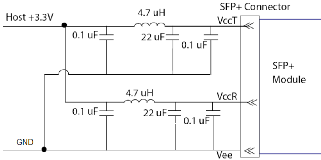
Рисунок 2. Host Board Power Supply Filters Circuit
