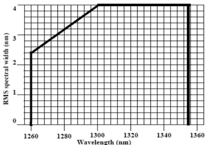
Figure 3 Transmitter Maximum RMS Spectral Width
