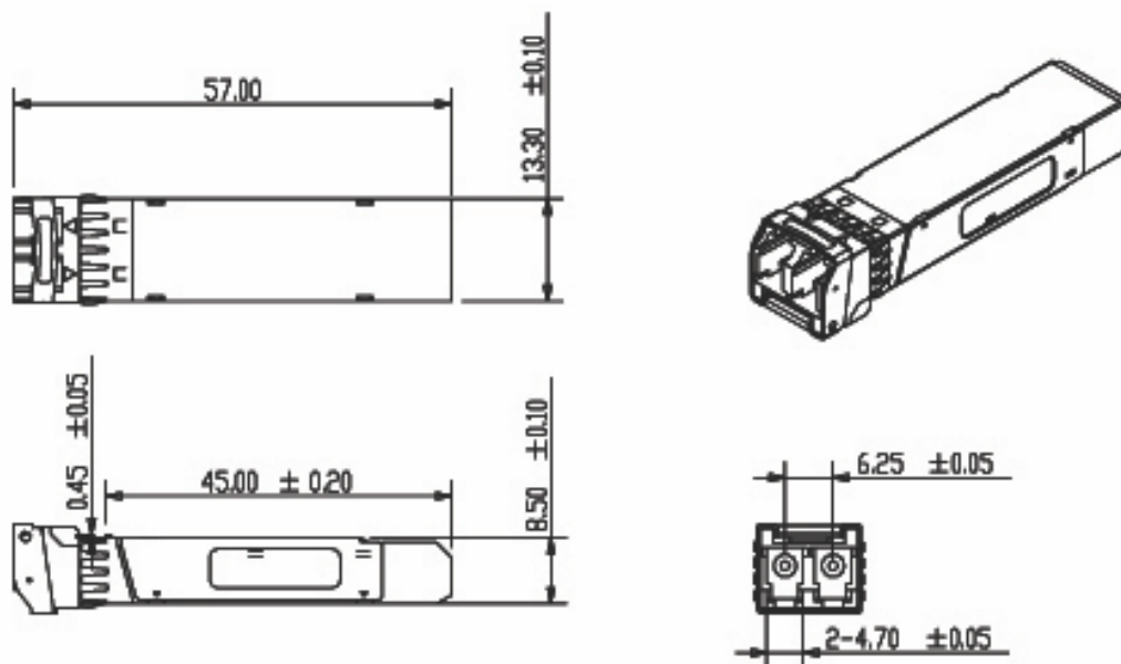
Figure4. Mechanical Specifications
