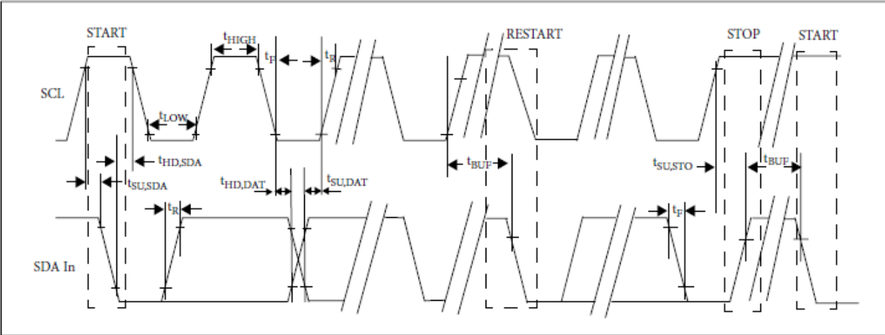
FIGURE 5-7 TIMING DIAGRAM
