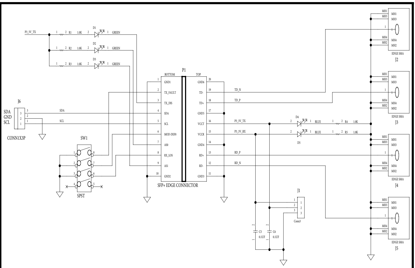
Figure 37 Schematic of the Host Compliance Board
